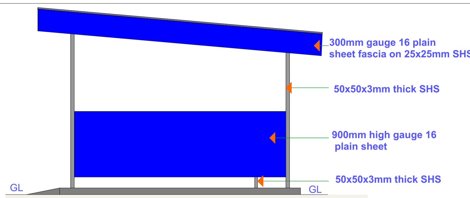
SIDE 01 ELEVATION
