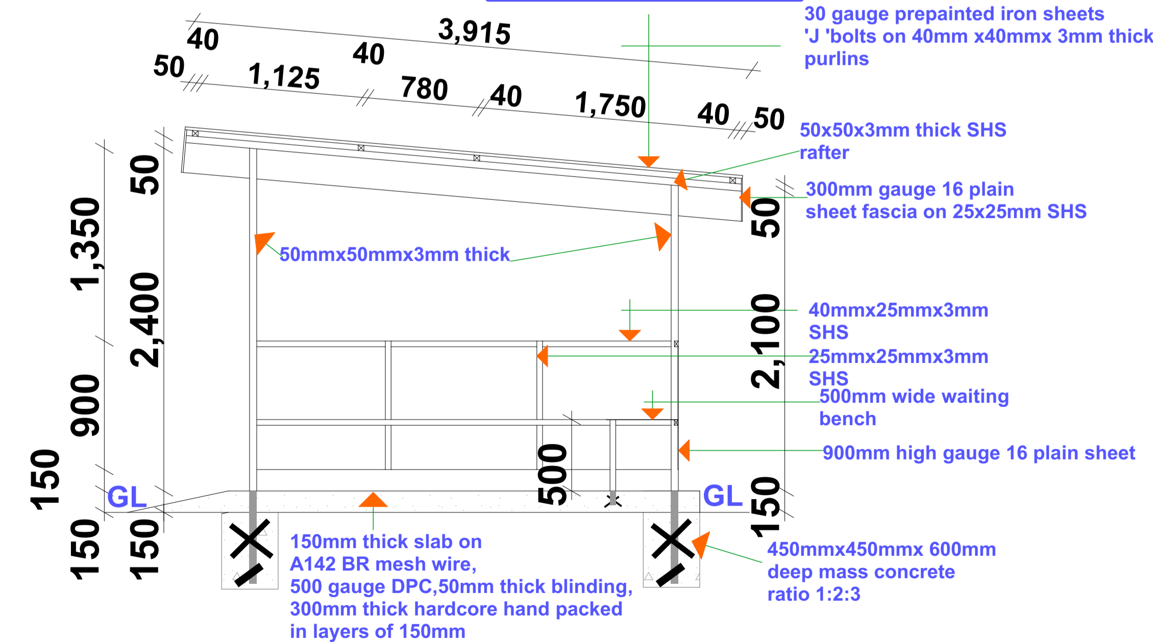
SECTION X
