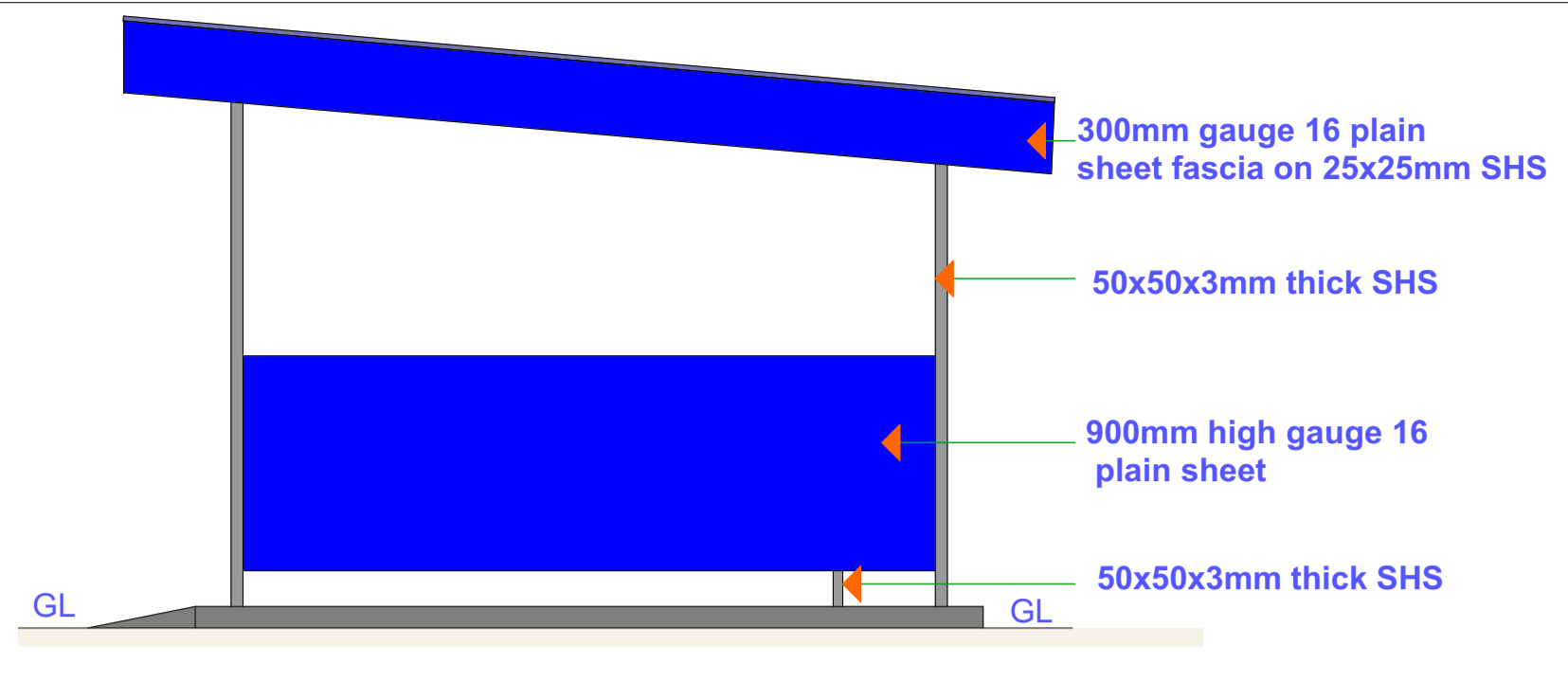
SIDE 01 ELEVATION
