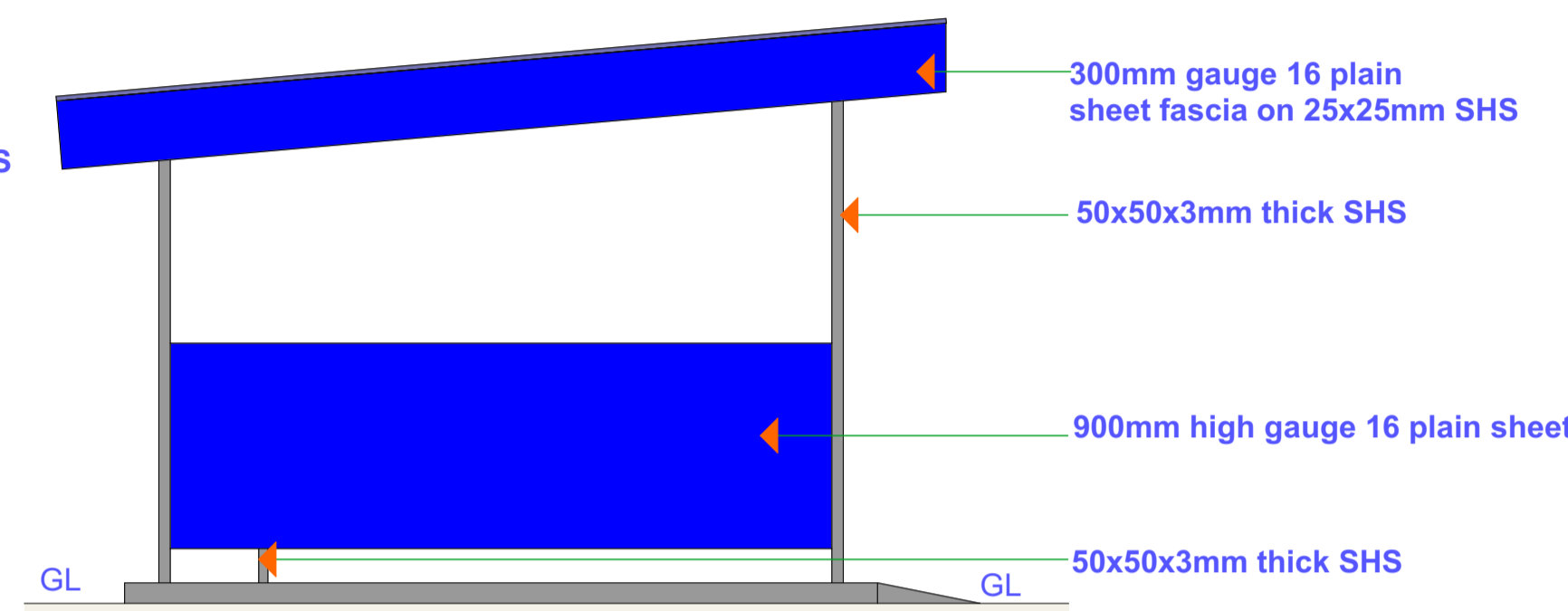
SIDE 02 ELEVATION
