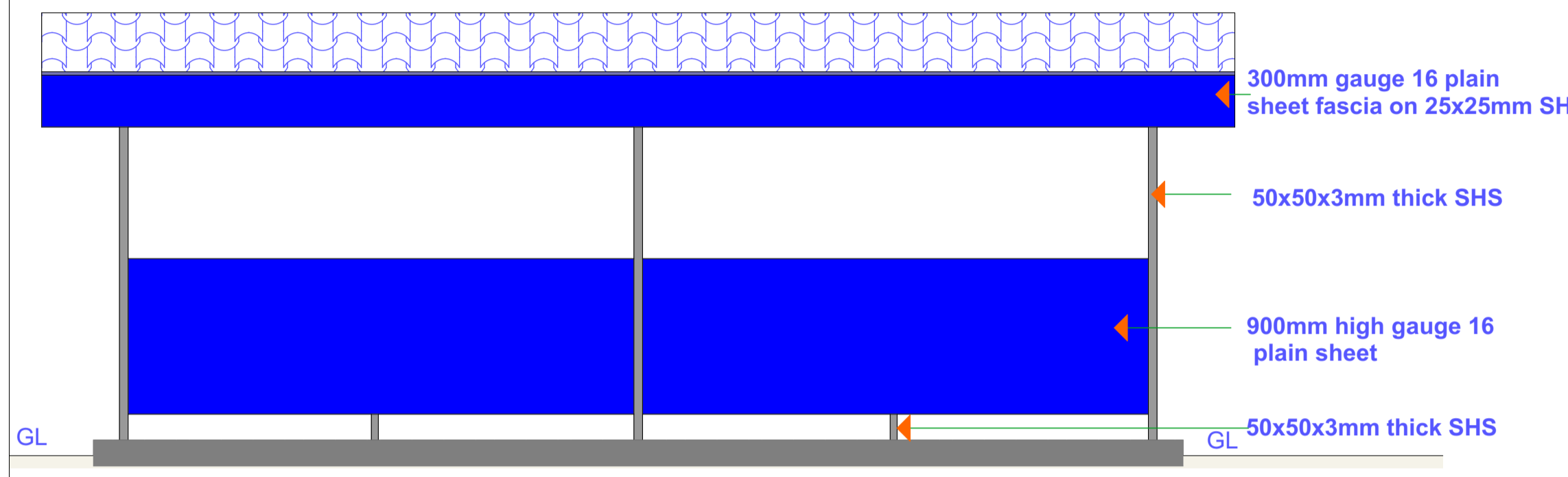
BACK ELEVATION
