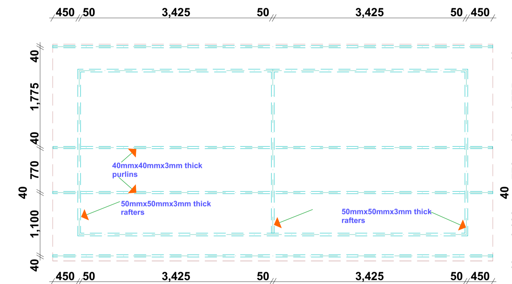
ROOF PLAN
