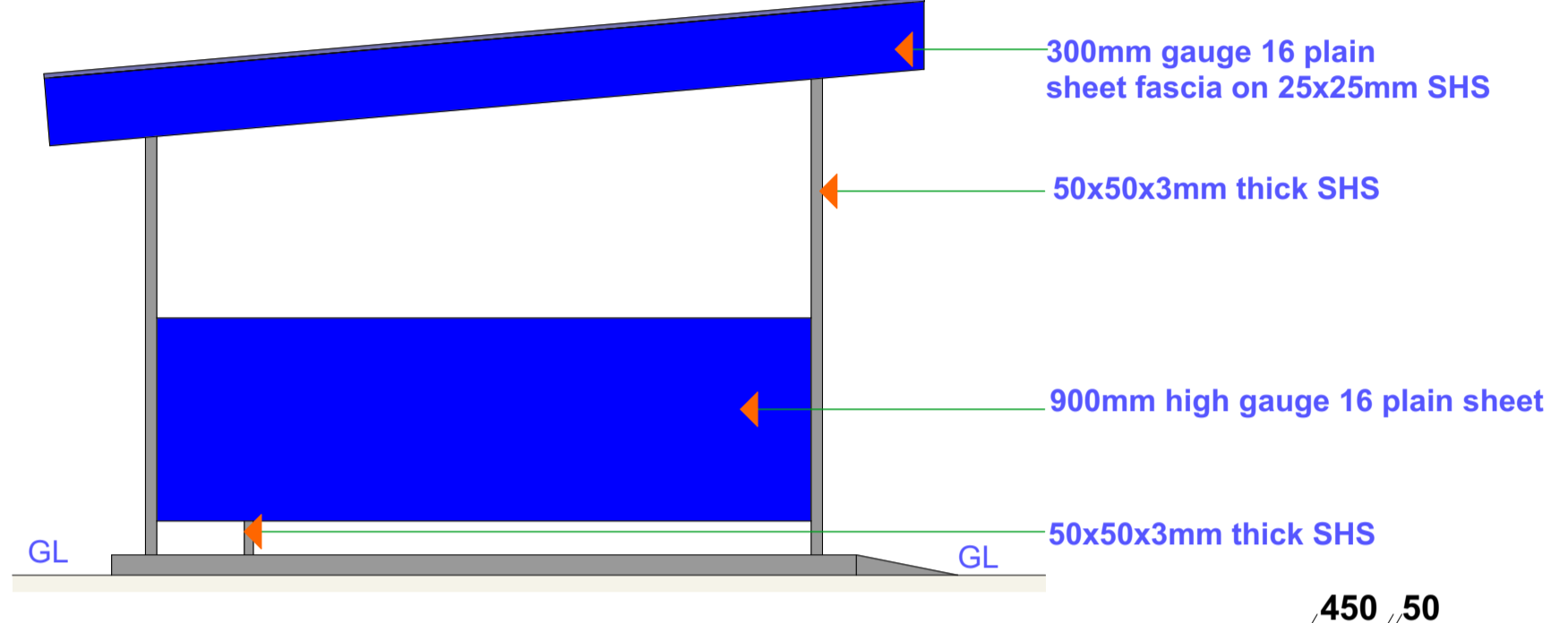
SIDE 02 ELEVATION
