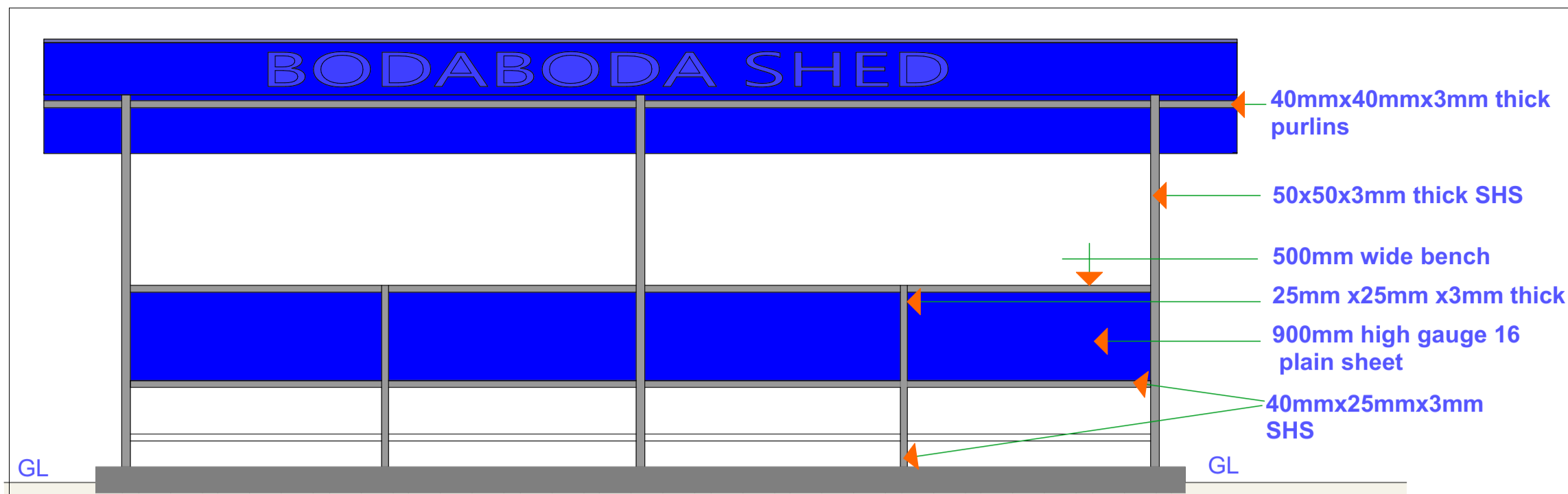
FRONT ELEVATION
