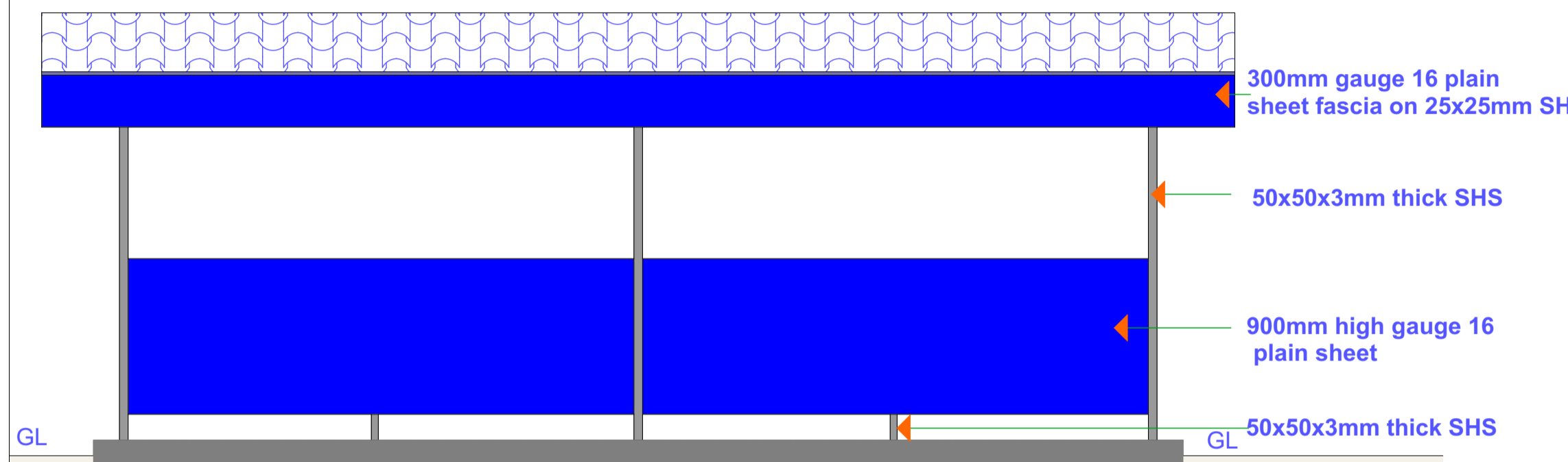
BACK ELEVATION
